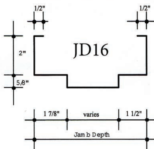
Typical Masonry Frame Profile
