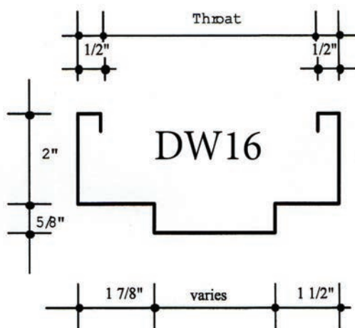
Typical Masonry Frame Profile
